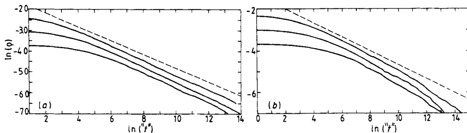
Figure 4. A+B \rightarrow O annihilation on percolation fractals. (a) d=2 square lattice [(1024)^2] sites for initial concentrations \rho_0 = 0.1, 0.05 and 0.025 at the percolation threshold p_c = 0.5927 . (b) d=3 sc lattice [(105)^3] sites for initial concentrations \rho_0 = 0.1, 0.05 and 0.02 at the percolation threshold p_c = 0.3117 . The broken lines indicate the lines of slope -\frac{1}{3} .
