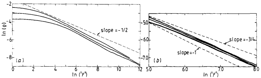
Figure 3. A + B \rightarrow O annihilation on Euclidean lattices. (a) d = 2 square lattice [(1024) 2 sites] for initial concentrations \rho_0 = 1.0, 0.05 and 0.025. (b) d = 3 sc lattice [(105) 3 sites] for initial concentrations \rho_0 = 1.0, 0.05 and 0.025.
