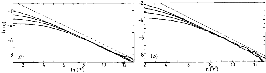
Figure 2. One-kind annihilation on percolation fractals ( A + A \rightarrow O ). (a) d = 2 square lattice [(1024) 2 sites] at the percolation threshold p_c = 0.5927 , for initial concentrations 0.2, 0.1, 0.05 and 0.025. (b) d = 3 sc lattice [(105) 3 sites] at the percolation threshold p_c = 0.3117 , for the same initial concentrations as in (a). Note that the limiting slope is independent of d ('superuniversal'). The broken lines have slope -2/5 .
